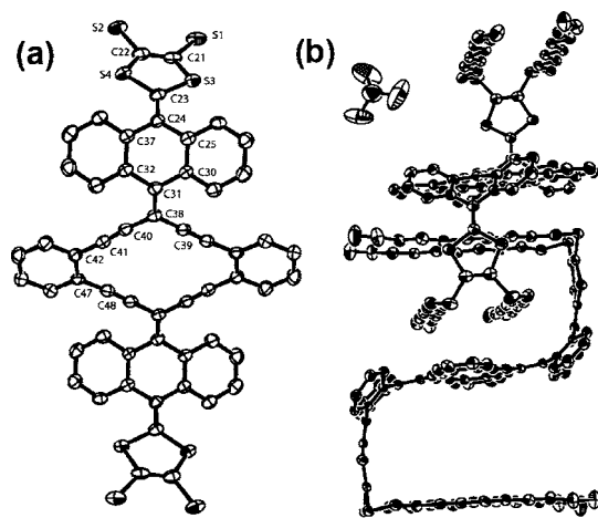
Figure 2. (a) ORTEP drawing of compound 1b at the 50% probability level ( n -decyl chains were removed for clarity). (b) Solid-state packing of two molecules of 1b in the unit cell. Selected bond lengths (Å): C23–C24 1.361(5), C24–C37 1.474(6), C32–C37 1.410(5), C31–C32 1.478(7), C31–C38 1.374(7), C38–C40 1.431(5), C40–C41 1.189(5), C41–C42 1.439(5), C42–C47 1.429(7). Selected bond angles (deg): C25–C24–C37 114.9(3), C30–C31–C32 113.8(4), C39–C38–C40 113.9(4), C38–C40–C41 174.3(6), C40–C41–C42 175.2(5), C41–C42–C47 121.1(4).
