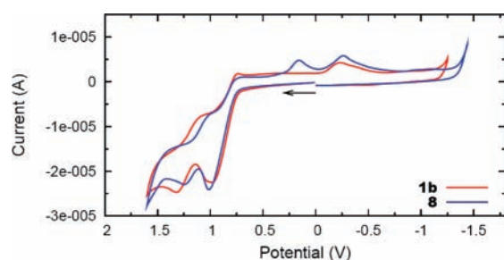
Figure 4. Cyclic voltammograms of 1b and 8 as measured in \text{CHCl}_3/\text{CH}_3\text{CN} (4:1, v/v) at room temperature. \text{Bu}_4\text{NBF}_4 (0.1 M) as the supporting electrolyte, glassy carbon as the working electrode, Pt wire as the counter electrode, and \text{Ag}/\text{AgCl} as the reference. Scan rate: 0.1\text{ V s}^{-1} .
