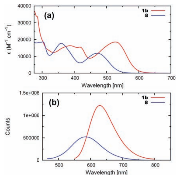
Figure 3. (a) UV–vis absorption spectra of 1b and 8 measured in CHCl 3 . (b) Fluorescence spectra of 1b ( \lambda_{\text{ex}} = 531 nm, \Phi = 0.13 ) and 8 ( \lambda_{\text{ex}} = 447 nm, \Phi = 0.064 ) measured in degassed CHCl 3 .
