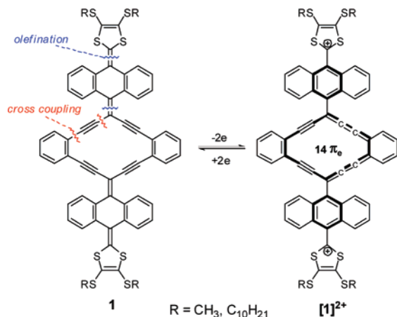
Figure 1. Molecular structures of compounds 1 in neutral and dicationic states.
