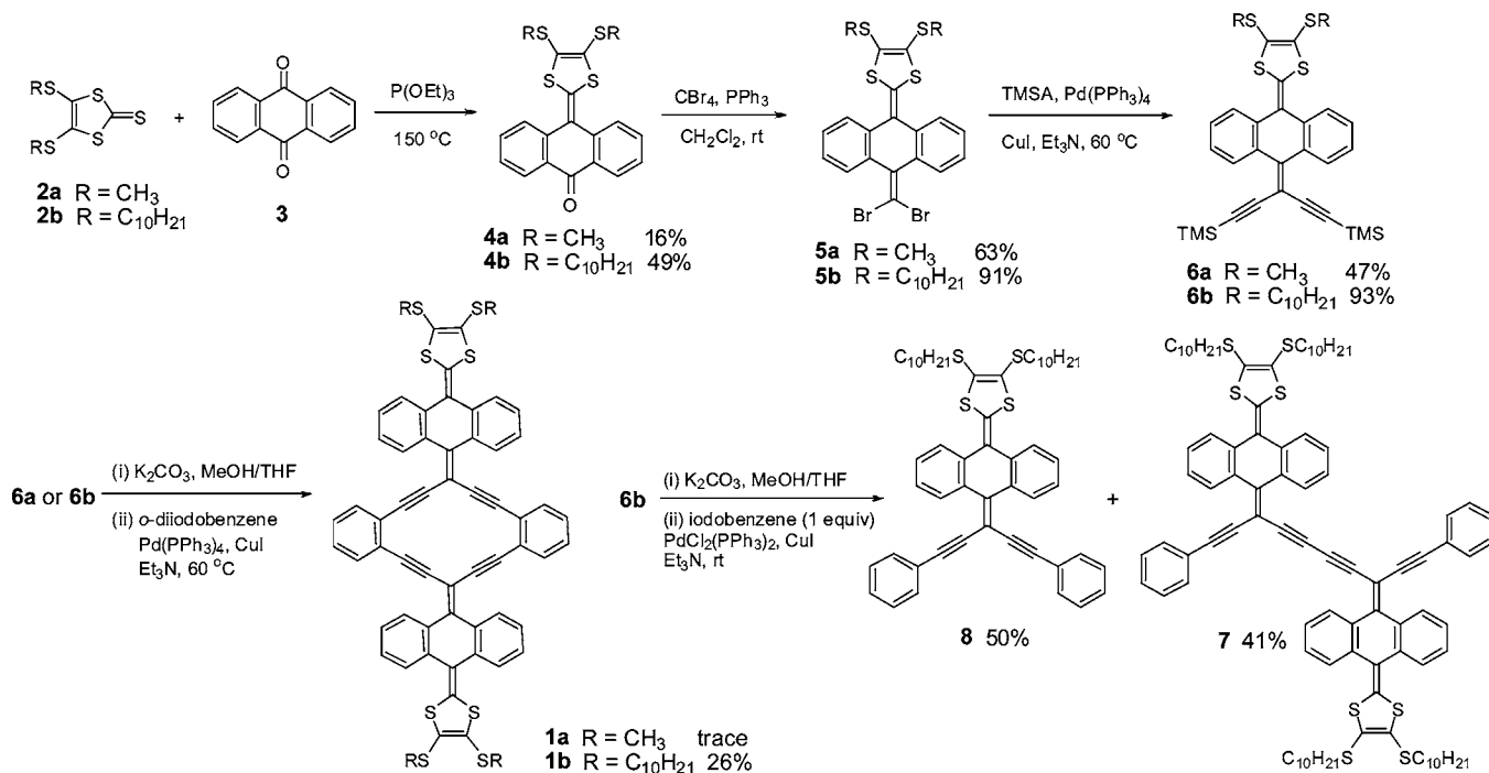
Scheme 1. Synthesis of exTTFs 1 and Reference Compound 8
